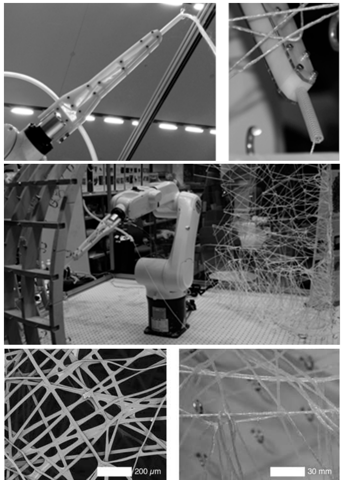
Figure 5. Fiber pulling tool (top), fiber pulling tool on KUKA robotic arm with external hook structure (middle), comparison of epoxy resin-soaked polypropylene twine (bottom right) and SEM image of scaffolding silk fiber (bottom left).
